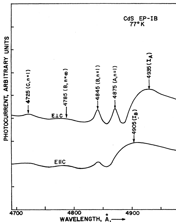
FIG. 3. Photoconductivity spectra of CdS at 77°K in polarized light.
