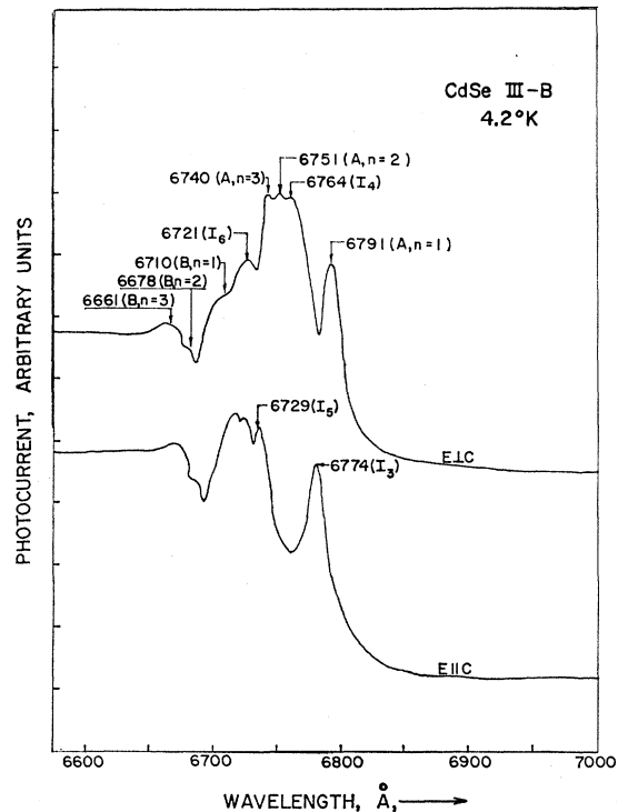
FIG. 6. Photoconductivity spectra of CdSe at 4.2°K in polarized light.
